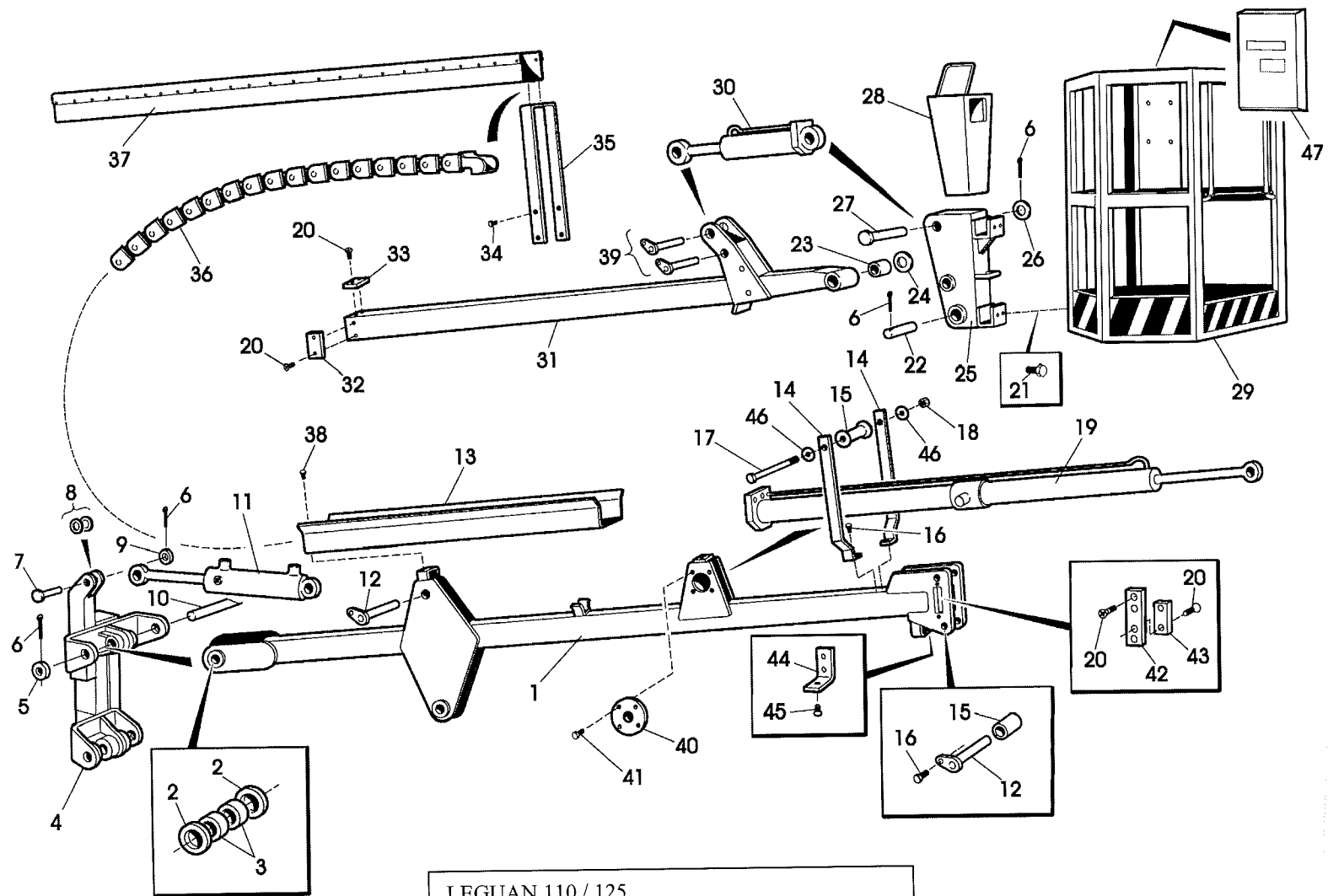
LEGUAN 110 / 125 DRAWING No. 5 UPPER BOOMS AND PLATFORM
