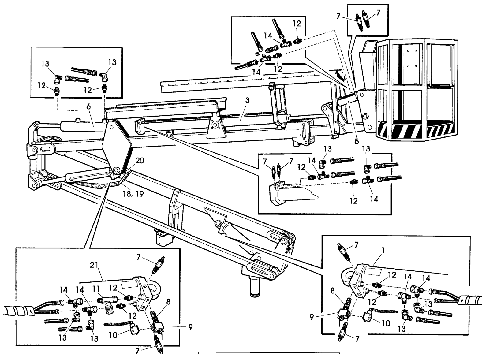
LEGUAN 110 / 125 DRAWING No. 3A CYLINDERS OF THE BOOM CONSTRUCTION
