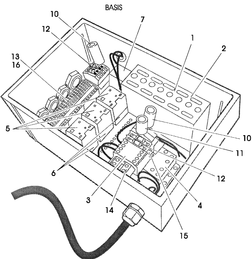
LEGUAN 110 / 125 DRAWING No. 10 ELECTRIC BOX
