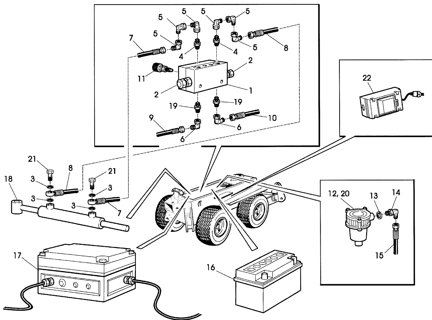
LEGUAN 110 / 125 DRAWING No. 8 SLEWING CYLINDER AND HOSE ASSEMBLY
