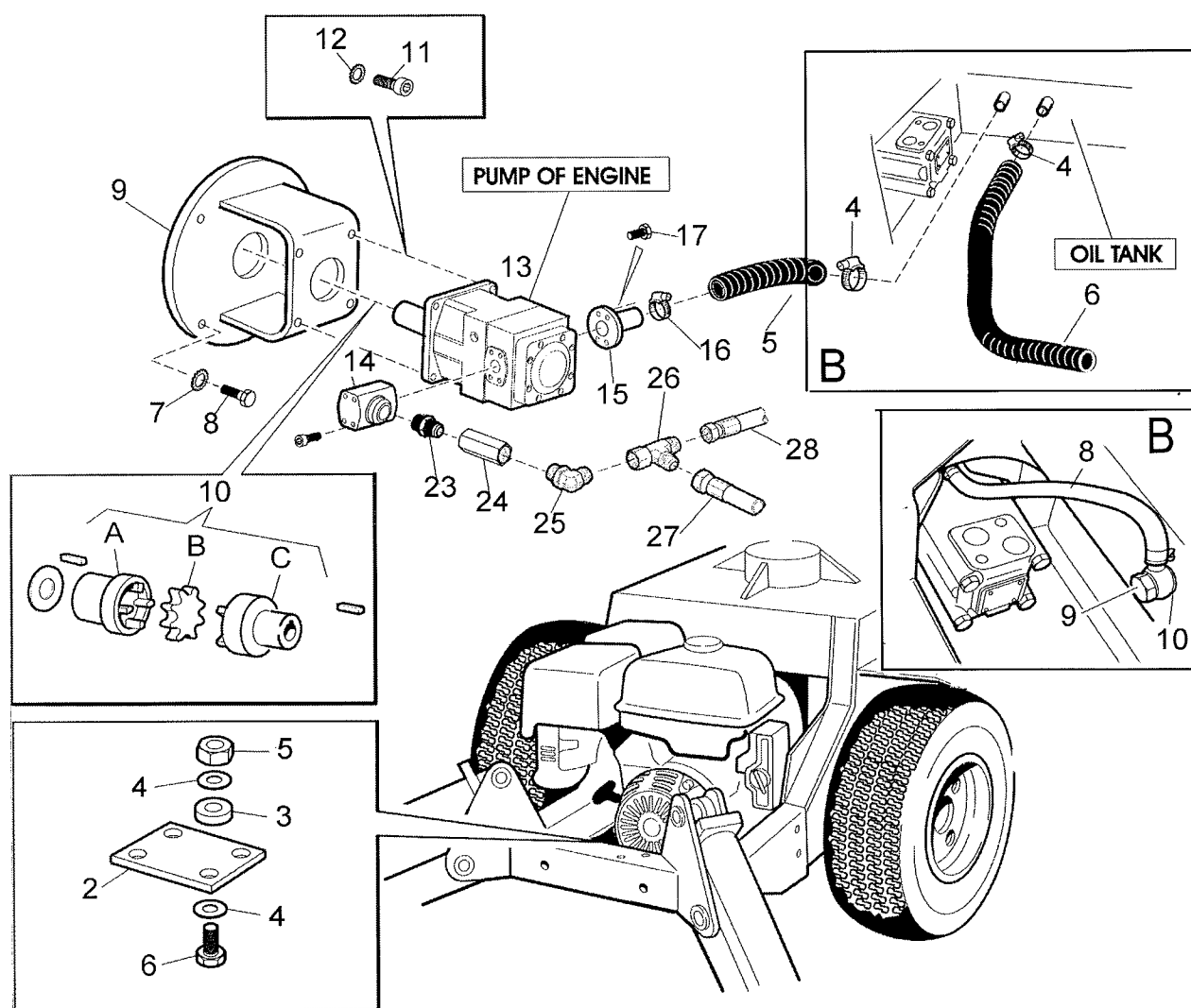
LEGUAN 110 / 125 DRAWING No. 2A+2B COUPLING, PUMP PRESSURE LINE AND INLET
