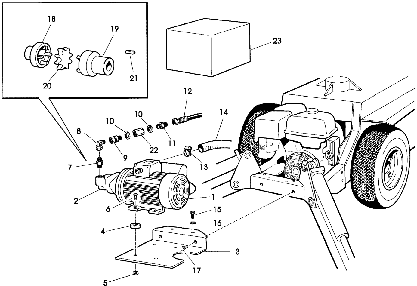
LEGUAN 110 / 125 DRAWING No. 9 110/230VAC PROPELLING UNIT ( OPTION)
