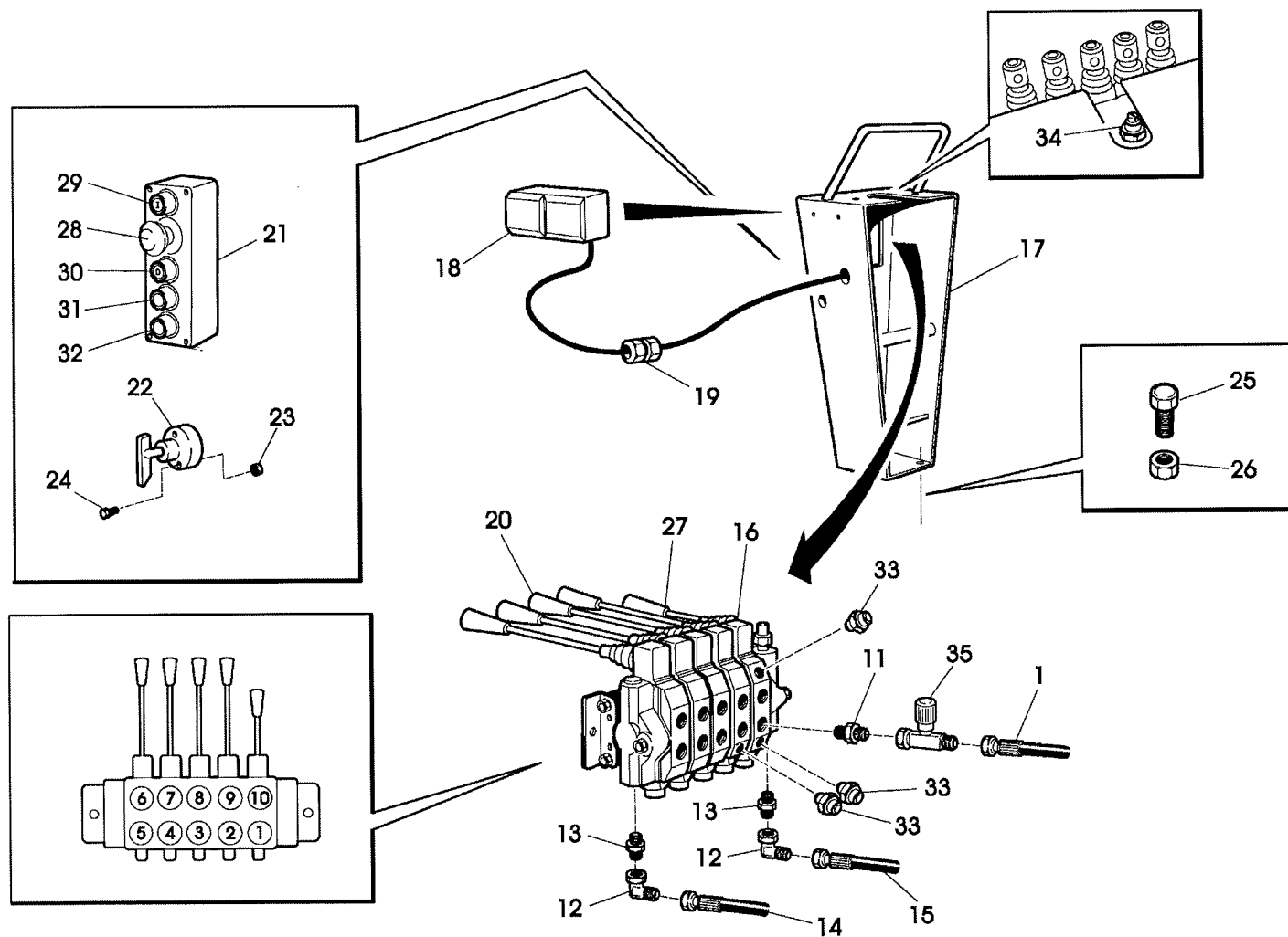
LEGUAN 110 / 125 DRAWING No. 7 UPPER CONTROL VALVE BLOCK AND HOSES
