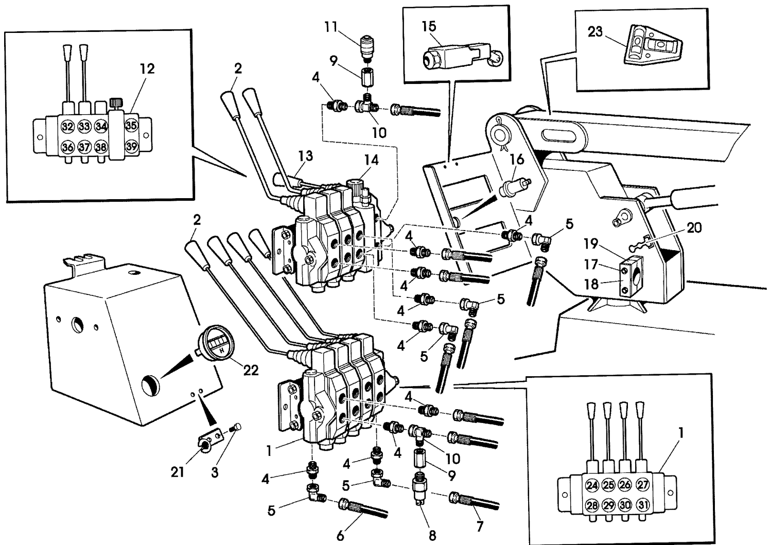
LEGUAN 110 / 125 DRAWING No. 6 OUTRIGGER CONTROL AND MAINDRIVE BLOCKS AND HOSES
