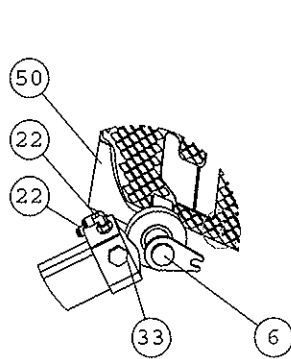
DETAIL F SCALE 1 : 10
